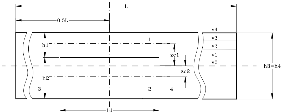
Fig. 1. The composite plate with delamination.
