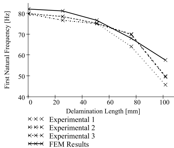
Fig. 3. The natural frequency of the loaded plate vs. experimental results [13] for L/h = 125 and various delamination lengths placed in vertical position 1.
