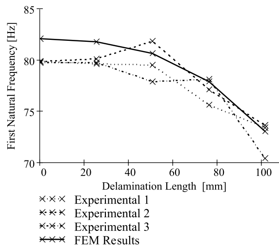
Fig. 4. The natural frequency of the loaded plate vs. experimental results [13] for L/h = 125 and various delamination lengths placed in vertical position 3.
