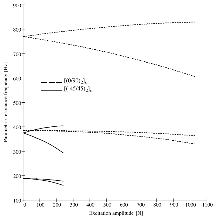
Fig. 13. The influence of the ply orientation on the instability regions, L/h = 25 .
