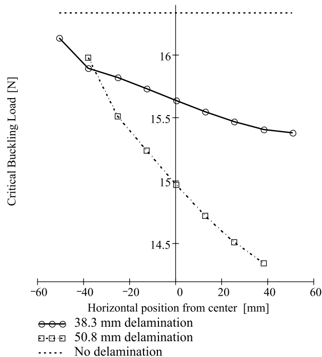
Fig. 10. The critical buckling load of the plate vs. the horizontal position of 38.3 and 50.8 mm mid-plane delaminations L/h = 125 .
