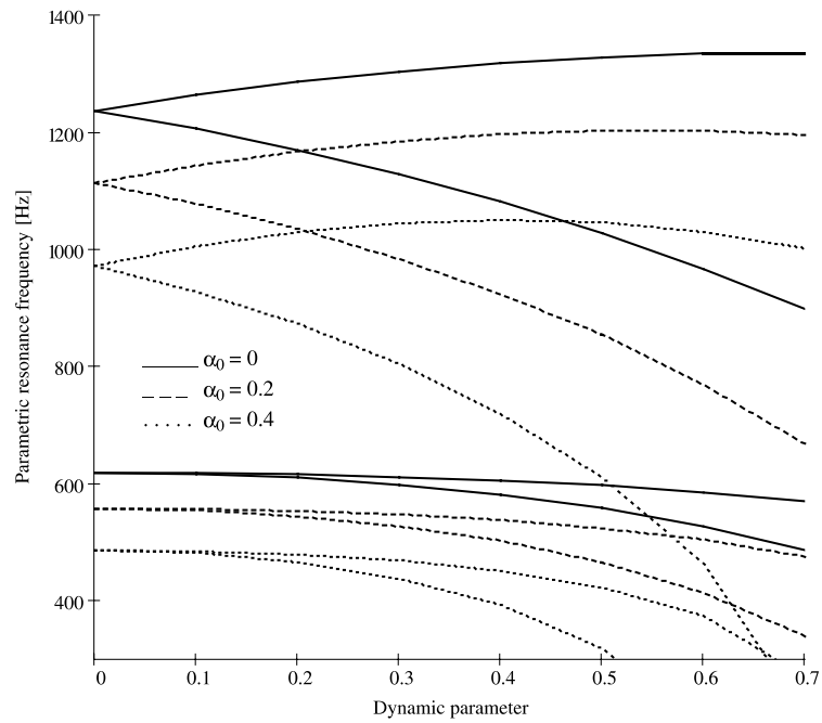
Fig. 11. The influence of the static component of the buckling force on the instability regions, L/h = 12.5 , 50.8 mm delamination.
