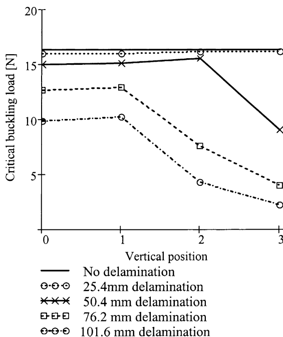
Fig. 6. Critical buckling load vs. vertical position for various delamination lengths.
