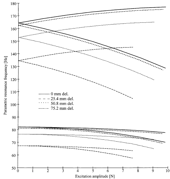
Fig. 12. The influence of the delamination length on the instability regions, L/h = 125 .
