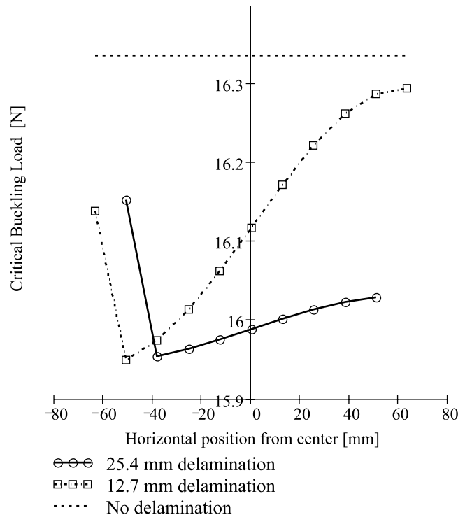
Fig. 9. The critical buckling load of the plate vs. the horizontal position of 12.7 and 25.4 mm mid-plane delaminations L/h = 125 .
