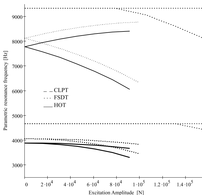
Fig. 2. The second order approximation of the instability regions for the three plate theories, L/h = 12.5 , case 2.
