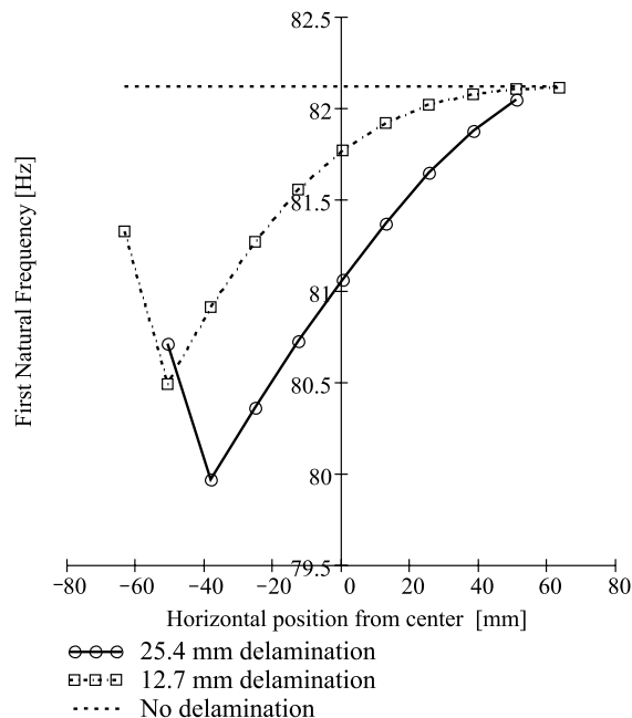
Fig. 8. The natural frequency of the plate vs. the horizontal position of 12.7 and 25.4 mm mid-plane delaminations, L/h = 12.5 .
