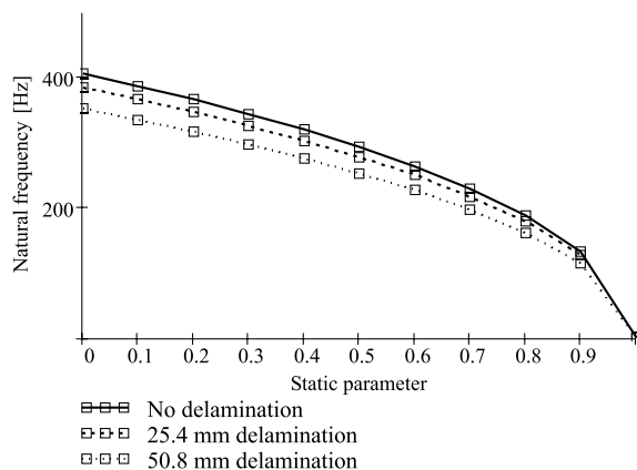
Fig. 5. The natural frequency of the loaded plate L/h = 25 .
