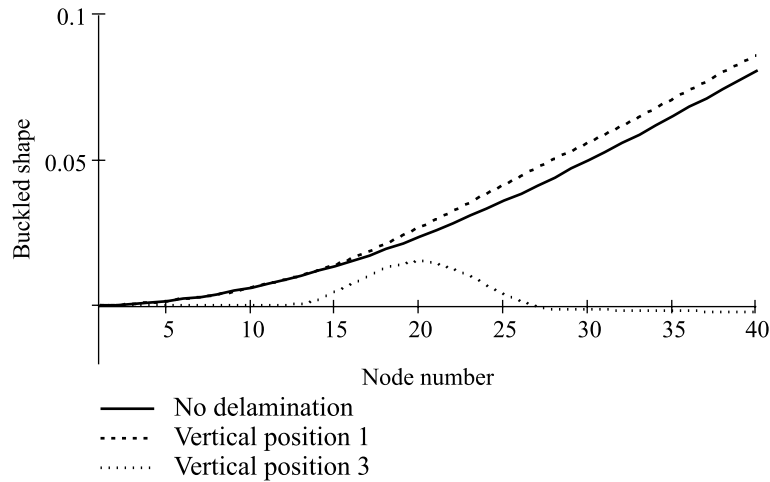
Fig. 7. The buckled shape of the plate for a 50.8 mm delamination and vertical position 0, 1 and 3.
